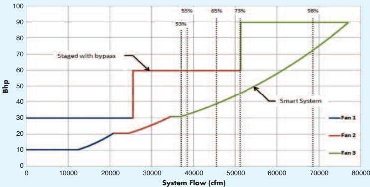
Model TS3S300D12 30hp (3 Fans Operating)
